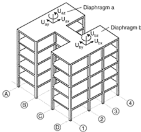
FIGURE 14.25 Independent rigid diaphragms linked by flexible elements.
