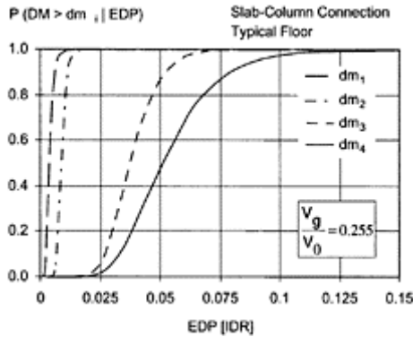
FIGURE 9.36 Fragility functions for four damage measures of slab-to-column connections representative of a flat plate in an existing seven-story reinforced concrete building.
