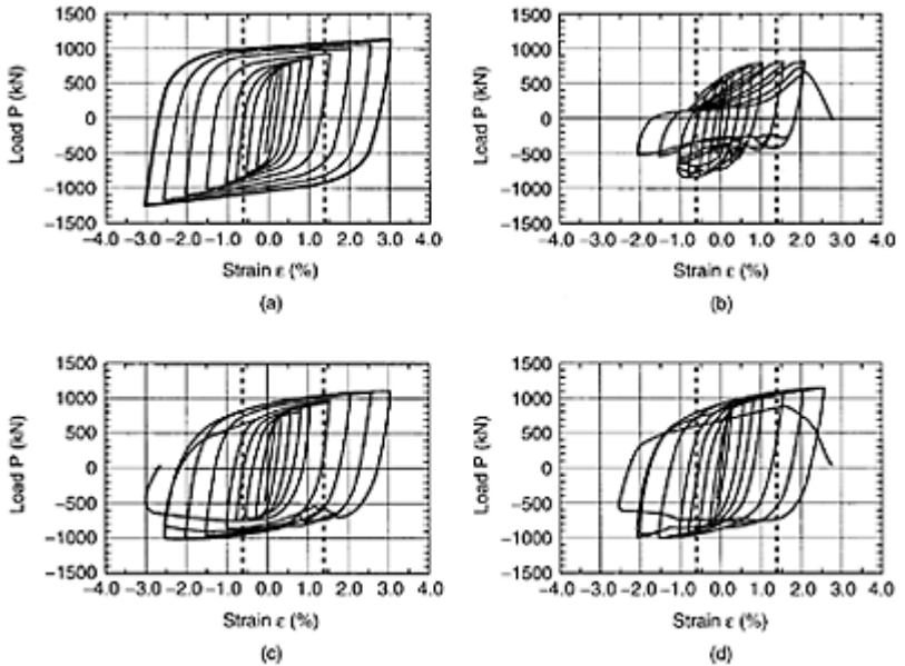
FIGURE 16.20 Cyclic response of four test specimens. (a) Type 1; (b) type 2; (c) type 3; (d) type 4. (Iwata, M., Kato, T. and Wada, A. (2000). Buckling-restrained braces as hysteretic dampers, Proc. STESSA , Quebec, PQ, pp. 33–38).
