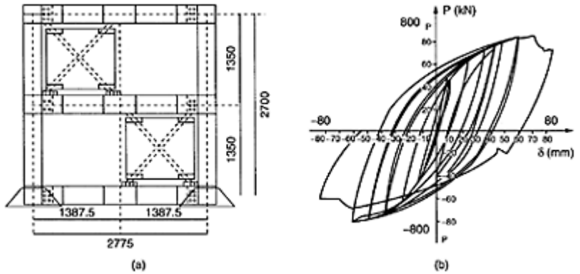
FIGURE 16.16 System test of budding-restrained braces sandwiched between precast concrete panels, (a) Test setup; (b) hysteresis behavior. (Wakabayashi, M., Nakamura, T., Kashibara, A., Morizono, T. and Yokoyama, H. (1973). Experimental study of elasto-plastic properties of precast concrete wall panels with built-in insulating braces, Summaries of Technical Papers of Annual Meeting , Architectural Institute of Japan, pp. 1041–1044 (in Japanese).)
