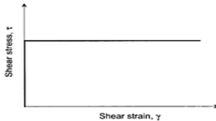
FIGURE 4.38 Stress-strain curve for rigid-perfectly plastic material, which is the assumed condition in limit equilibrium slope stability analyses.
