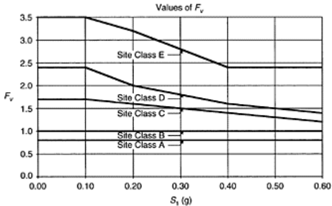
FIGURE 14.8 Values of F_v as a function of site class and S_1 .
