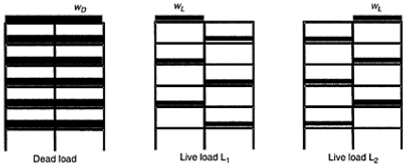
FIGURE 14.14 Distributed gravity (dead and live) loads acting on the girders of the frame.
