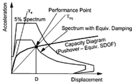
FIGURE 9.6 Illustration of capacity spectrum method.
