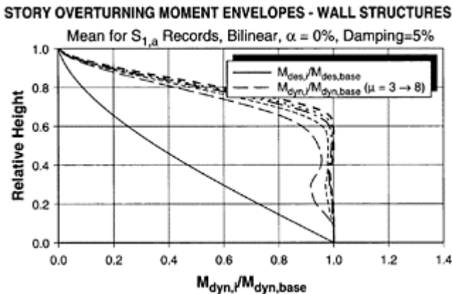
FIGURE 9.15 Story overturning moments for a wall structure with T=2.05 sec. (Seneviratna, G.D.RK. and
