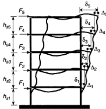
FIGURE 14.16 Story drift computation.
