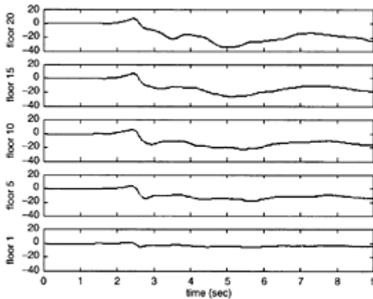
FIGURE 6.29 Displacement history (in inches) at five floor levels in 20-story building due to horizontal ground acceleration.
