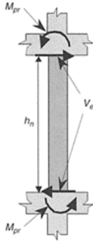
FIGURE 14.33 Calculation of V_e for columns.
