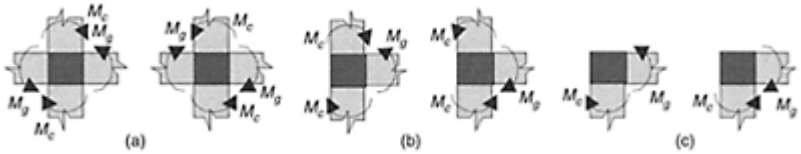
FIGURE 14.30 Minimum flexural strength of columns.
