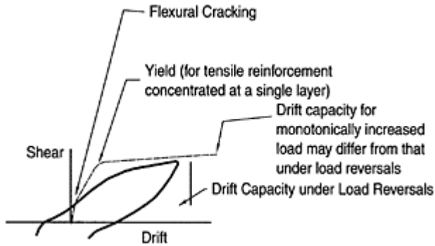
FIGURE 13.20 Drift capacity.
