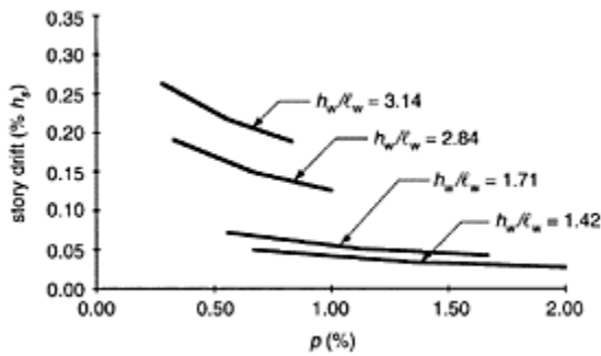
FIGURE 14.48 Story drift as a percentage of story height obtained for different values of the wall area ratio, p , for eight-story building having the plan layouts shown in Figures 14.46 and 14.47 and located in a moderate seismic zone studied in (Garcia, 1996).
